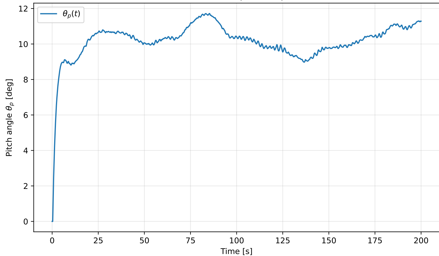
Turbulent wind: pitch response
